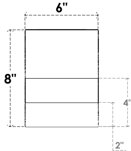
FRONT PROFILE
